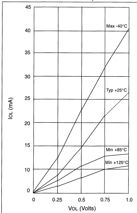
FIGURE 12-10: IOL vs. VOL, VDD = 3.5 V
