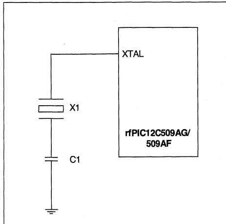
FIGURE 7-2: EXAMPLE ASK EXTERNAL CRYSTAL CIRCUIT
