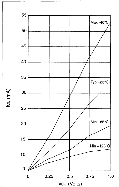
FIGURE 12-12: IOL vs. VOL, VDD = 5.5 V
