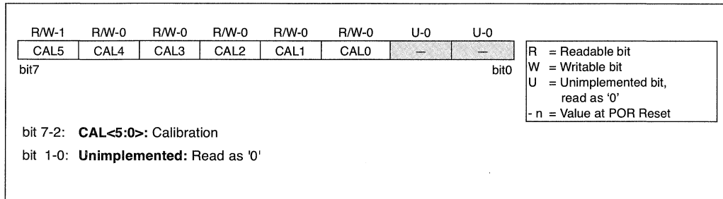
FIGURE 4-5: OSCCAL REGISTER (ADDRESS 05h)
