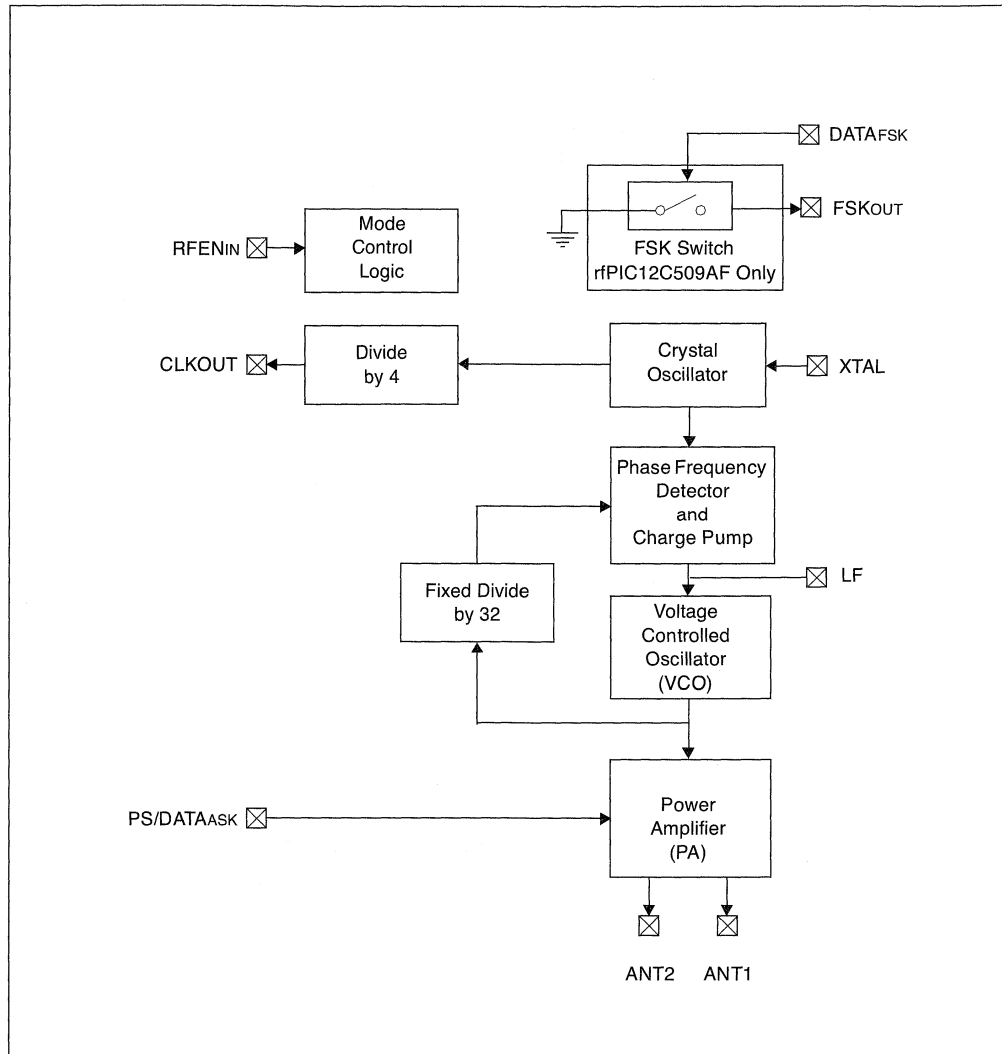
FIGURE 7-1: rfPIC12C509AG/509AF TRANSMITTER BLOCK DIAGRAM
