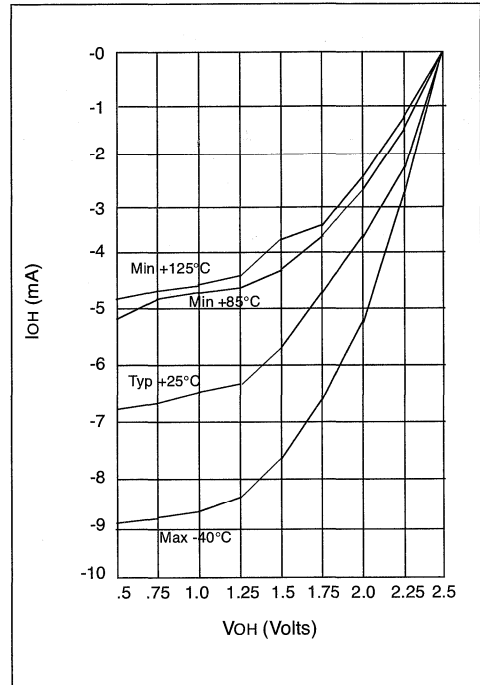
FIGURE 12-8: IOH vs. VOH, VDD = 3.5 V
