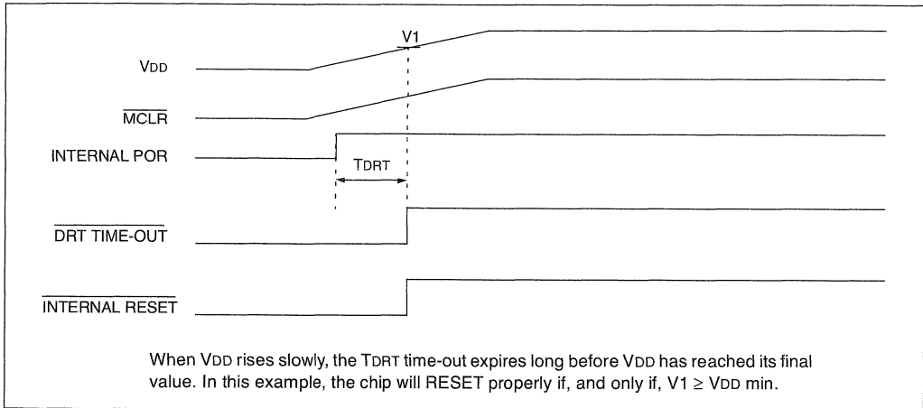
FIGURE 8-9: TIME-OUT SEQUENCE ON POWER-UP (MCLR TIED TO VDD): SLOW VDD RISE TIME
