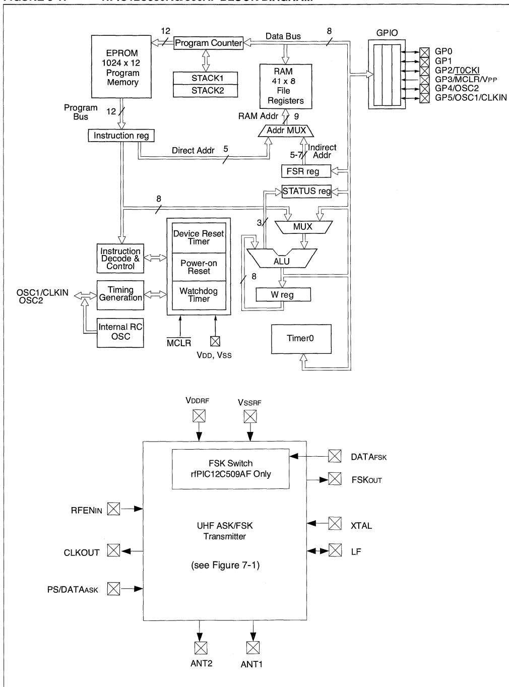
FIGURE 3-1: rfPIC12C509AG/509AF BLOCK DIAGRAM
