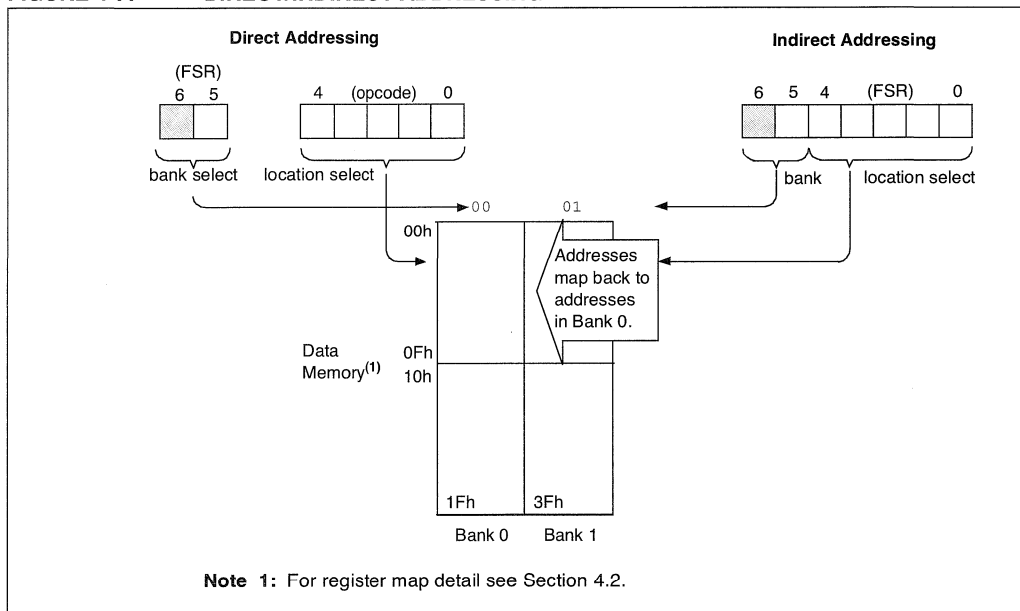
FIGURE 4-7: DIRECT/INDIRECT ADDRESSING
