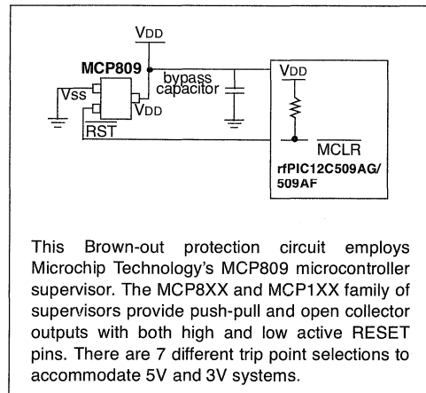
FIGURE 8-13: BROWN-OUT PROTECTION CIRCUIT 3
