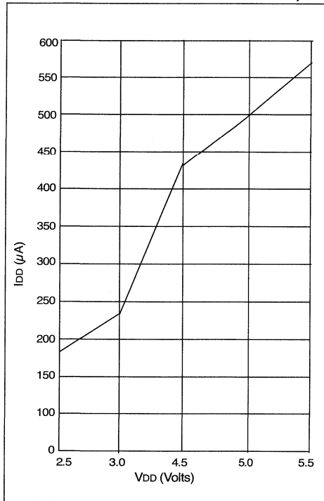
FIGURE 12-3: TYPICAL I DD VS. V DD (WDT DIS, 25°C, FREQUENCY = 4MHz)
