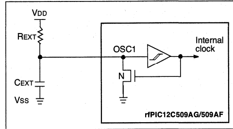
FIGURE 8-4: EXTERNAL RC OSCILLATOR MODE
