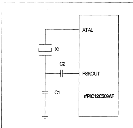
FIGURE 7-3: EXAMPLE FSK EXTERNAL CRYSTAL CIRCUIT
