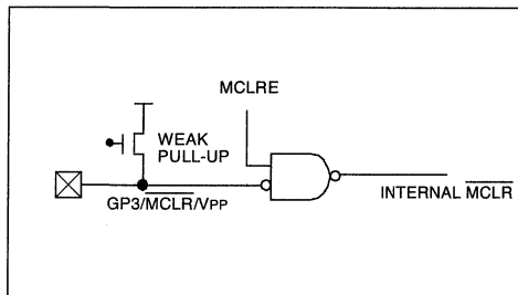
FIGURE 8-5: \overline{\text{MCLR}} SELECT
