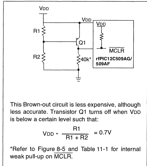
FIGURE 8-12: BROWN-OUT PROTECTION CIRCUIT 2
