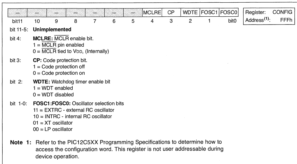
FIGURE 8-1: CONFIGURATION WORD FOR rfPIC12C509AG/509AF
