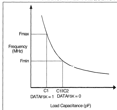
FIGURE 7-4: LOAD CAPACITANCE VERSUS CHANGE IN TRANSMITTED FREQUENCY
