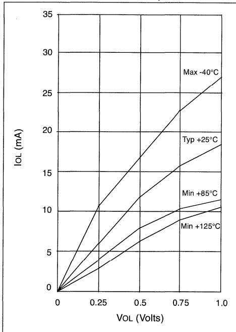
FIGURE 12-10: IOL vs. VOL, VDD = 3.5 V
