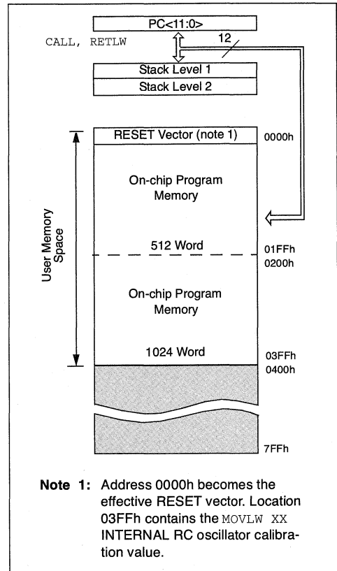
FIGURE 4-1: PROGRAM MEMORY MAP AND STACK
