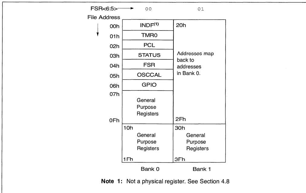
FIGURE 4-2: rfPIC12C509AG/509AF REGISTER FILE MAP
