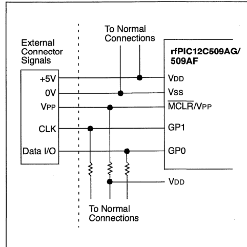
FIGURE 8-14: TYPICAL IN-CIRCUIT SERIAL PROGRAMMING CONNECTION
