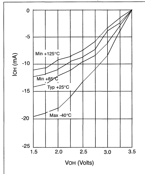
FIGURE 12-8: IOH vs. VOH, VDD = 3.5 V
