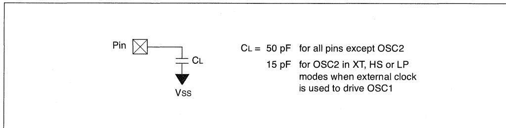
FIGURE 11-3: LOAD CONDITIONS
