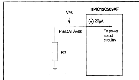
FIGURE 7-7: EXAMPLE FSK POWER SELECT CIRCUIT
