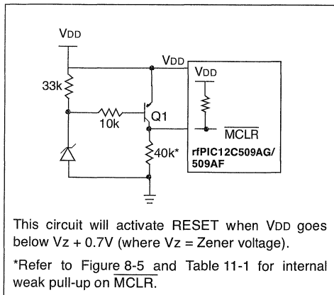
FIGURE 8-11: BROWN-OUT PROTECTION CIRCUIT 1
