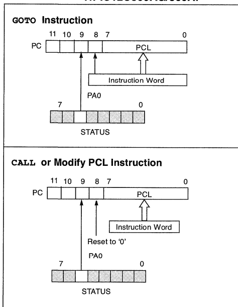
FIGURE 4-6: LOADING OF PC BRANCH INSTRUCTIONS - rPIC12C509AG/509AF
