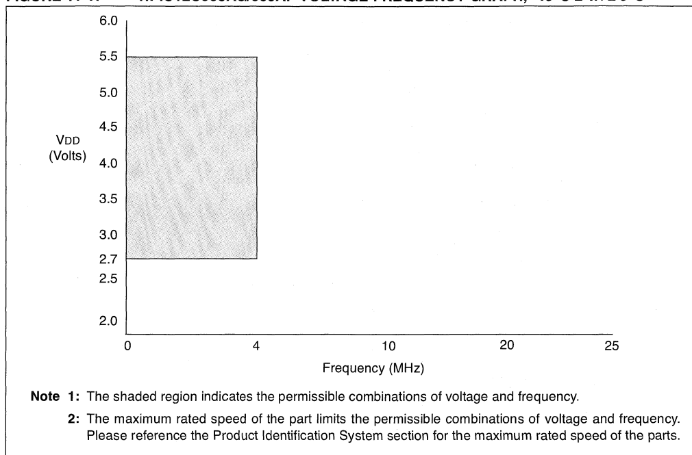
FIGURE 11-1: rfPIC12C509AG/509AF VOLTAGE-FREQUENCY GRAPH, -40^{\circ}\text{C} \leq T_A \leq 0^{\circ}\text{C}
