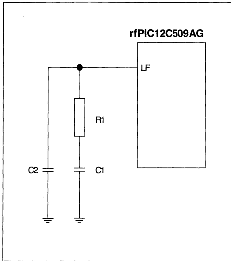
FIGURE 7-5: EXAMPLE LOOP FILTER CIRCUIT
