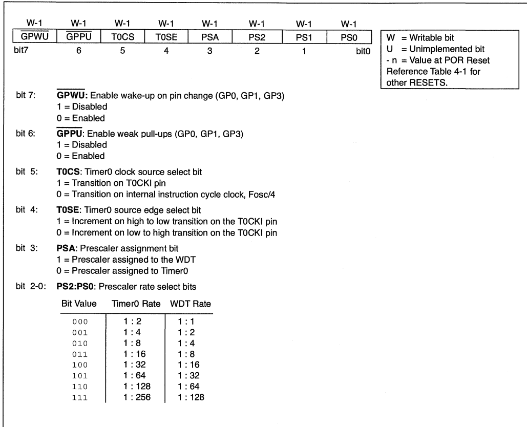
FIGURE 4-4: OPTION REGISTER
